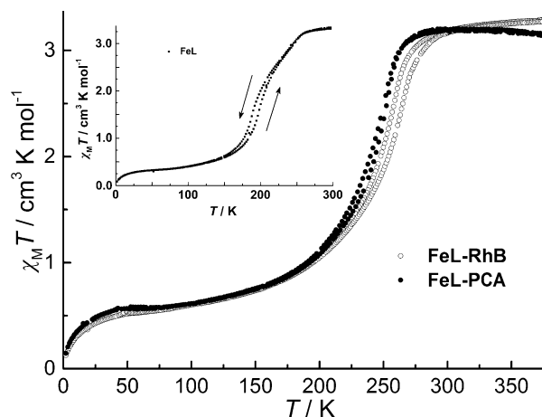
Figure 3. \chi_M T versus T plot of FeL-PCA and FeL-RhB at a sweep rate of 1 \text{ K min}^{-1} under an applied magnetic field of 5000 Oe. Inset: the magnetic properties of the as-synthesized FeL.
